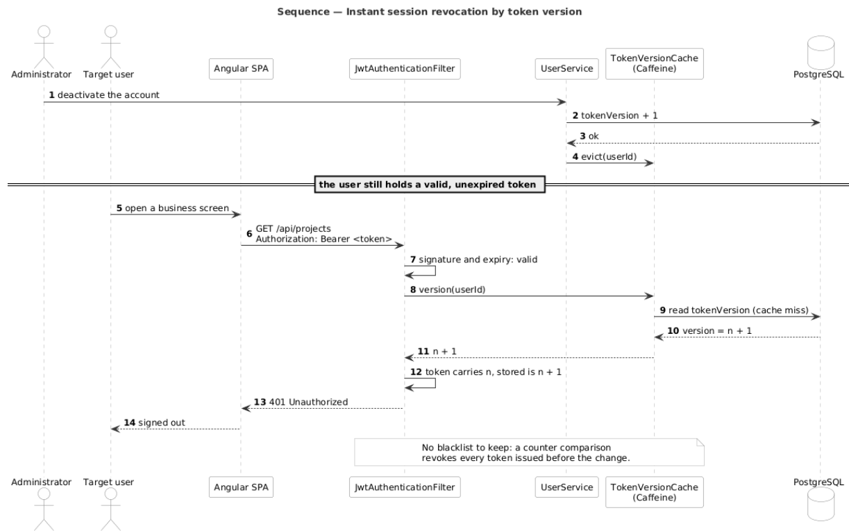
Figure 4.9: Sequence diagram of the “Revoke a session” use case
