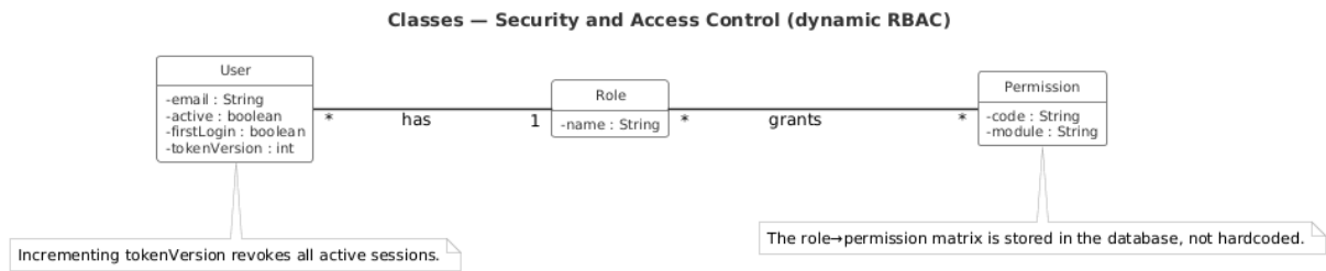
Figure 3.6: Class diagram — security and access control
