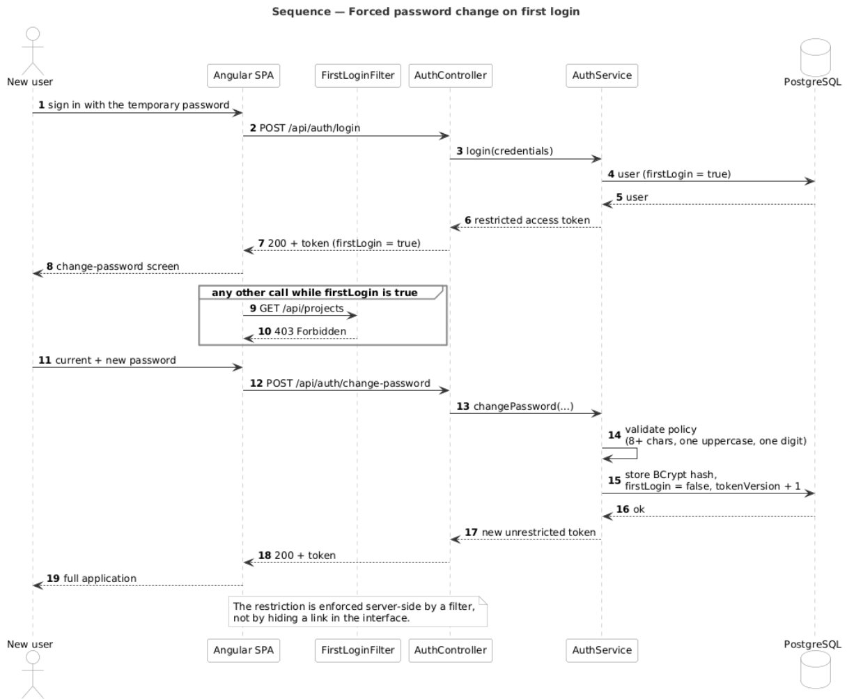
Figure 4.8: Sequence diagram of the “Change the password on first login” use case
