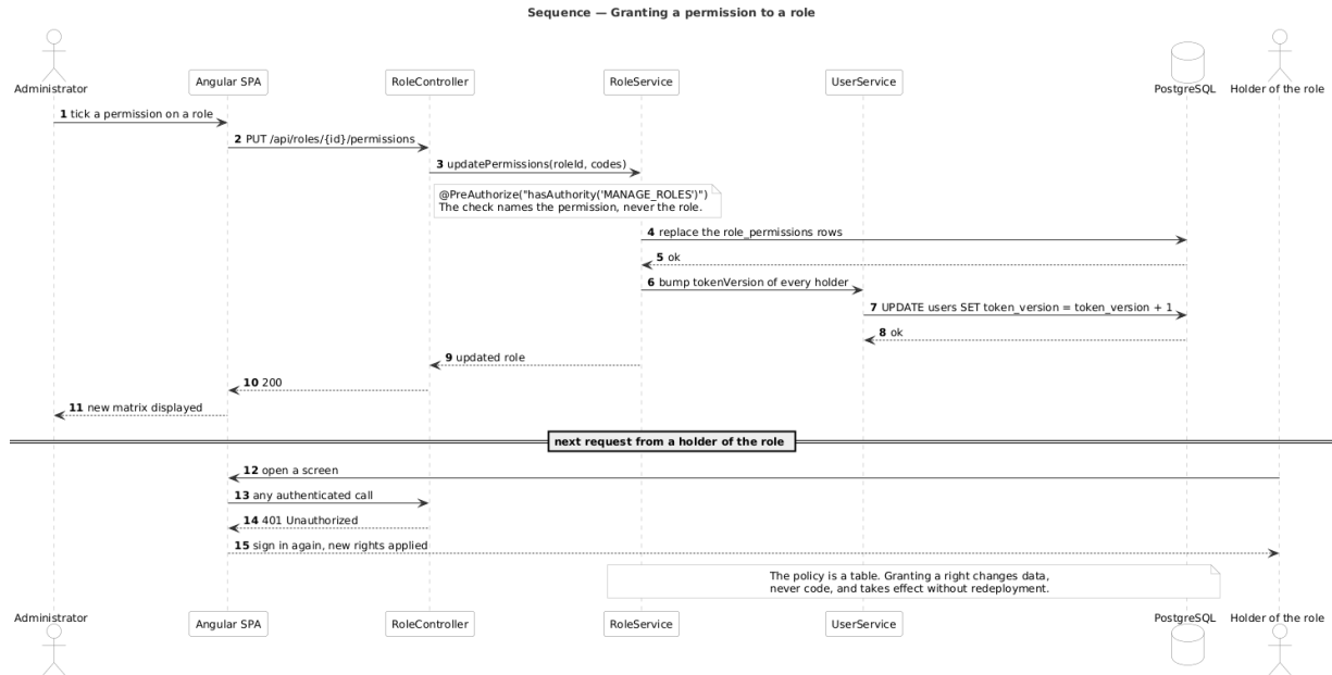
Figure 4.14: Sequence diagram of the “Grant a permission to a role” use case
