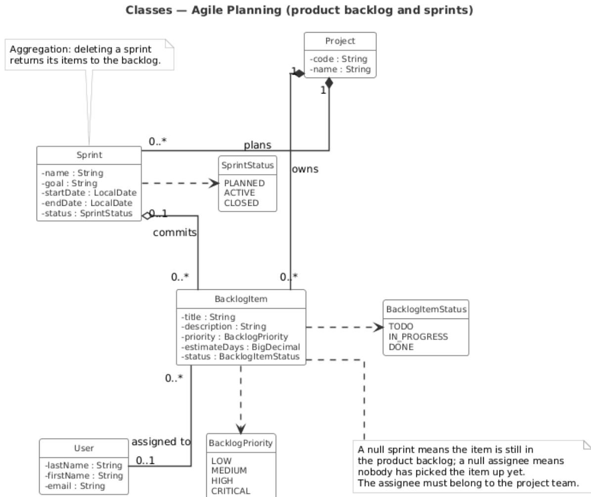
Figure 5.12: Class diagram — agile planning
