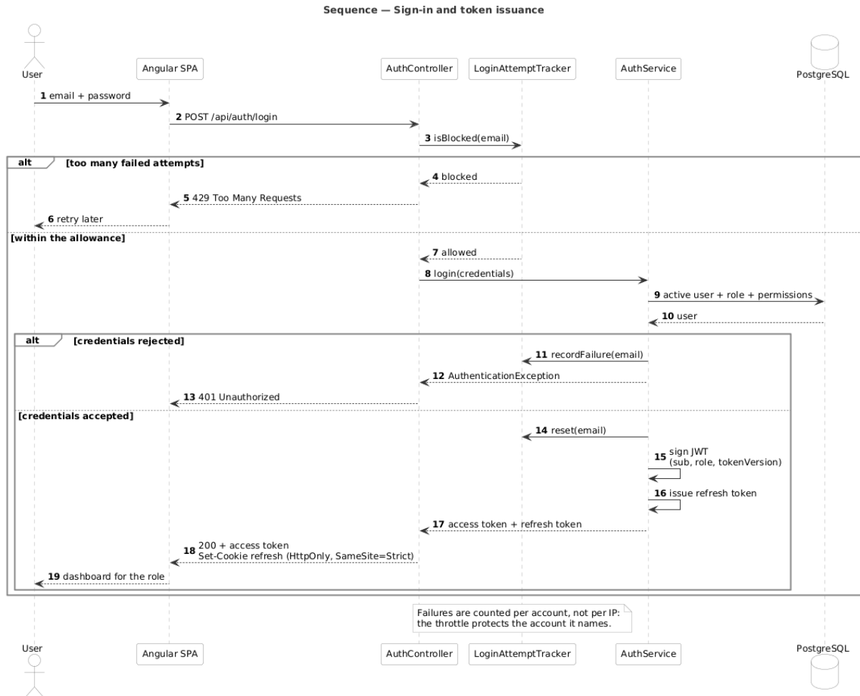
Figure 4.7: Sequence diagram of the “Authenticate” use case
