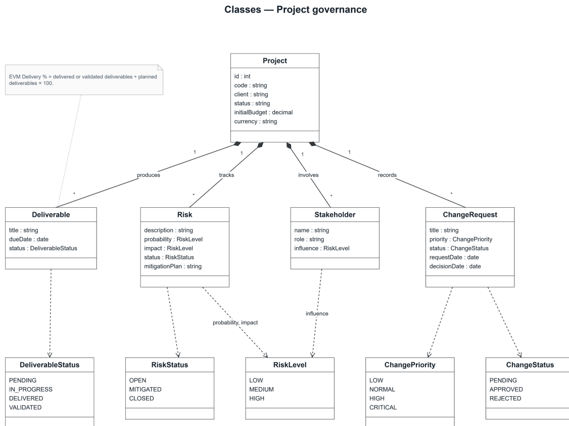
Figure 6.6: Class diagram — project governance
