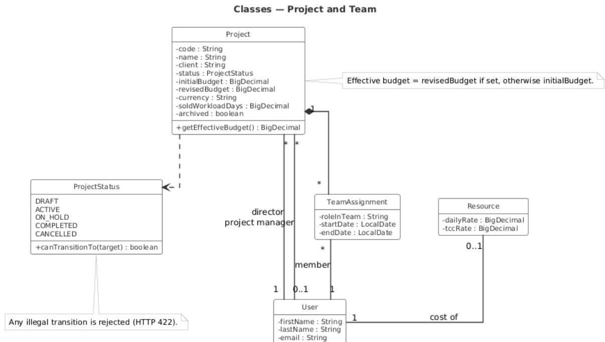
Figure 5.2: Class diagram — projects and teams
