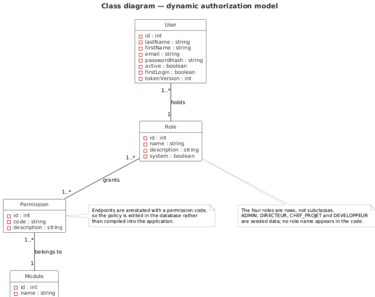
Figure 4.13: Class diagram of the authorization model
