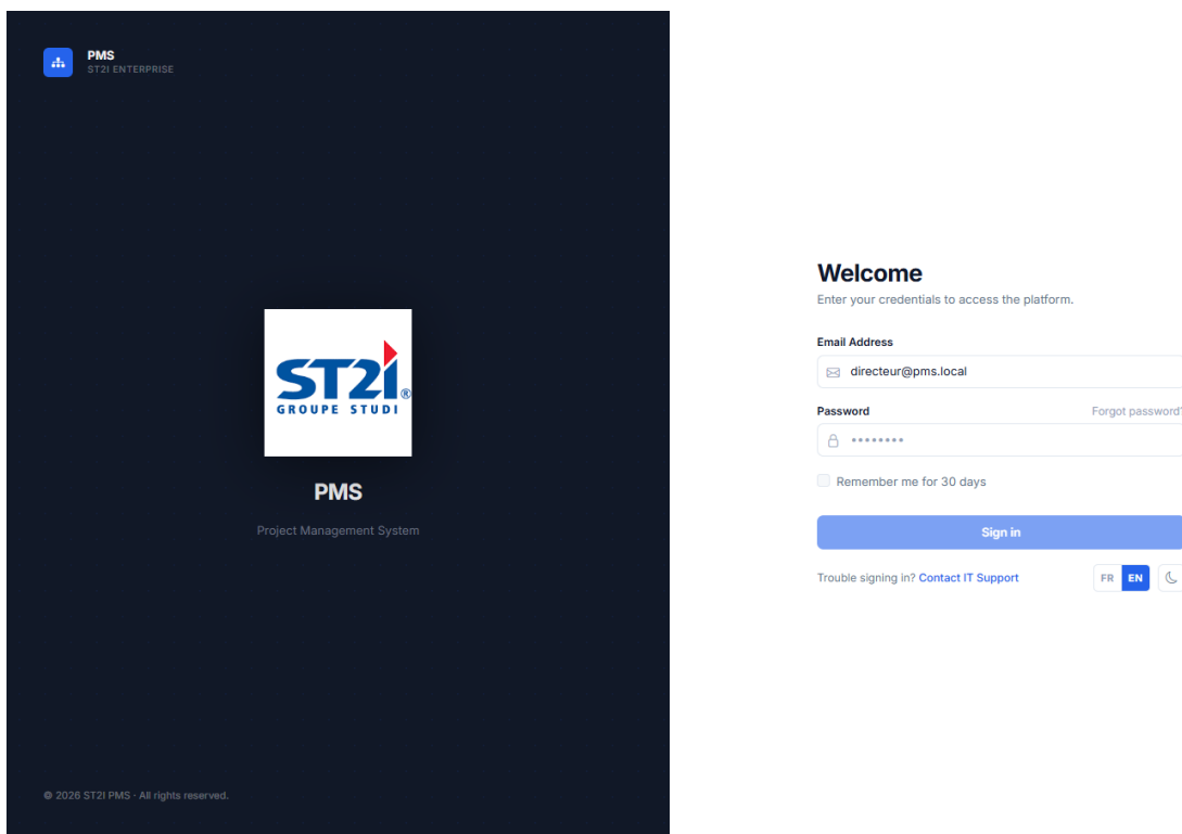
Figure 4.10: Login interface
