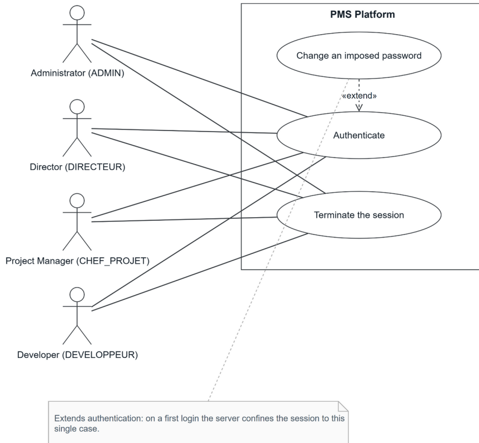
Figure 4.6: Use case diagram of sprint 1
