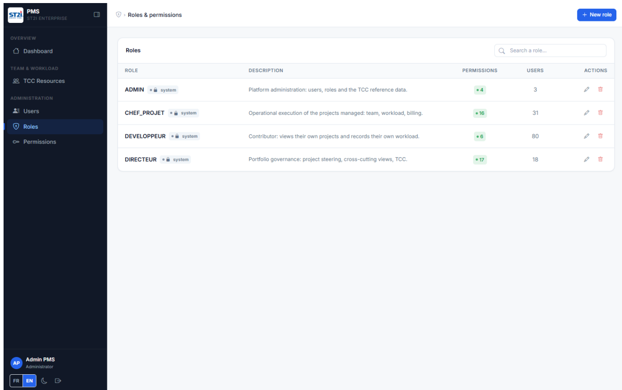
Figure 4.19: Role and permission management interface
